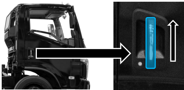
OPENING DOOR FROM OUTSIDE
